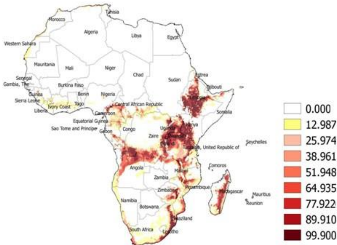
Figure 3. Projected Suitability of MCMV and potential risk of MLN across Africa by 2020, using Agro-ecological Niche Modelling*
